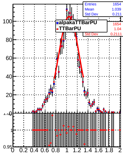
Jet response (pT/pTgen) in 28 \leq p_t < 37, 0.0 \leq |\eta| < 0.5
