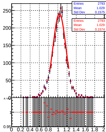
Jet response (pT/pTgen) in 64 <= pt < 84, 0.5 <= |eta| < 1.3
