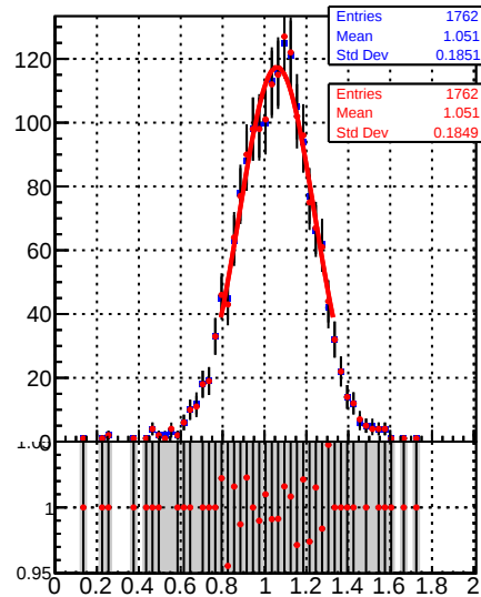
Jet response (pT/pTgen) in 64 <= pt < 84, 1.3 <= |eta| < 2.1
