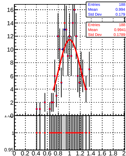
Jet response (pT/pTgen) in 64 <= pt < 84, 3.0 <= |eta| < 5.0
