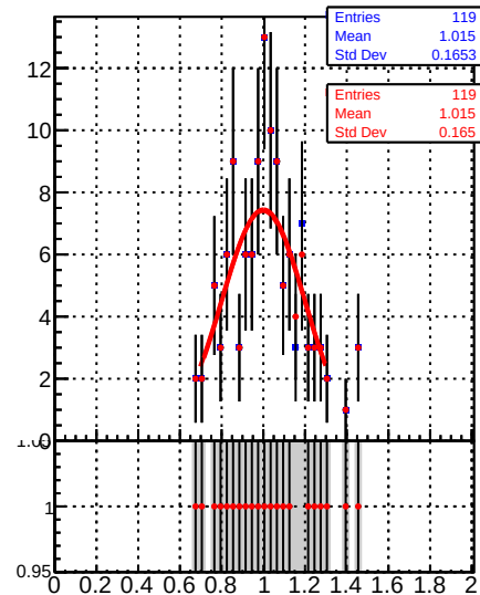
Jet response ( p_T/p_{T\text{gen}} ) in 84 \leq p_t < 114 , 3.0 \leq |\eta| < 5.0
