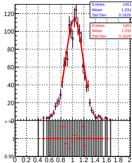
Jet response ( p_T/p_{T\text{gen}} ) in 84 \leq p_t < 114 , 1.3 \leq |\eta| < 2.1
