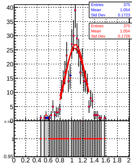
Jet response ( p_T/p_{T\text{gen}} ) in 84 \leq p_t < 114 , 2.1 \leq |\eta| < 2.5
