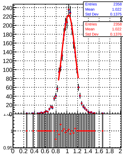
Jet response ( p_T/p_{T\text{gen}} ) in 84 \leq p_t < 114 , 0.5 \leq |\eta| < 1.3
