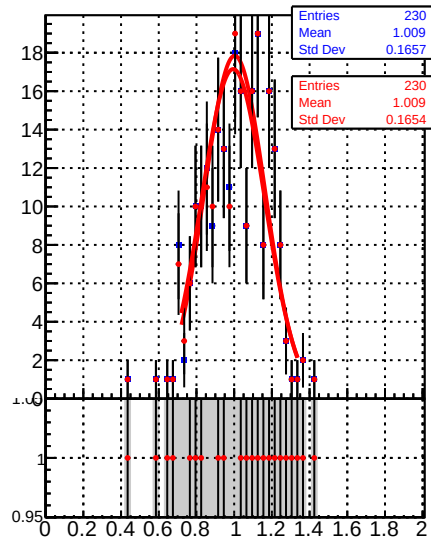
Jet response ( p_T/p_{T\text{gen}} ) in 84 \leq p_t < 114 , 2.5 \leq |\eta| < 3.0
