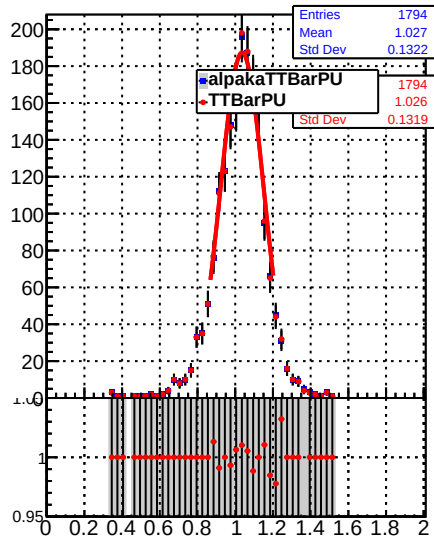
Jet response ( p_T/p_{T\text{gen}} ) in 84 \leq p_t < 114 , 0.0 \leq |\eta| < 0.5
