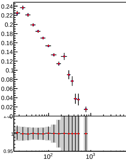
Raw Jet pT resolution using RMS, 1.3 < |\eta| < 2.1
