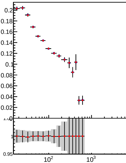
Raw Jet pT resolution using RMS, 0.5 < |\eta| < 1.3
