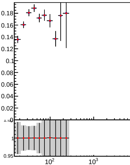
Raw Jet pT resolution using RMS, 3.0 < |\eta| < 5.0
