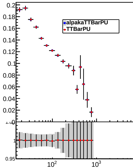
Raw Jet pT resolution using RMS, 0.0 < |\eta| < 0.5
