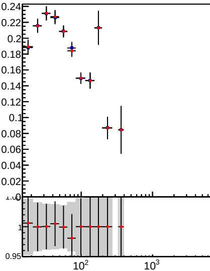
Raw Jet pT resolution using RMS, 2.5 < |\eta| < 3.0
