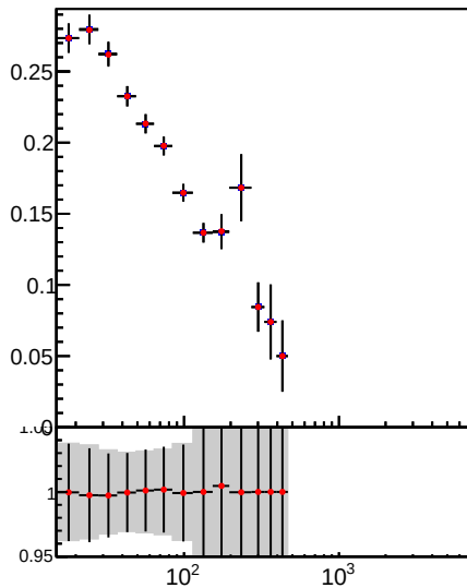
Raw Jet pT resolution using RMS, 2.1 < |\eta| < 2.5
