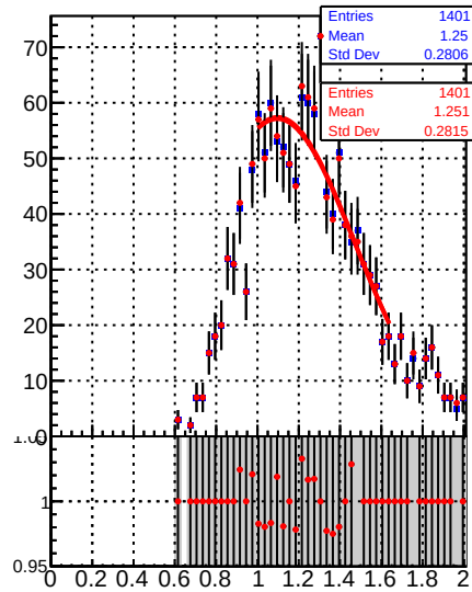
Raw Jet response (pT/pTgen) in 15 \leq p_t < 21, 1.3 \leq |\eta| < 2.1
