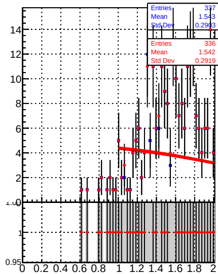
Raw Jet response (pT/pTgen) in 15 \leq p_t < 21, 2.5 \leq |\eta| < 3.0
