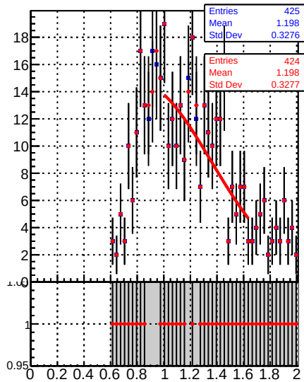
Raw Jet response (pT/pTgen) in 15 \leq p_t < 21, 2.1 \leq |\eta| < 2.5
