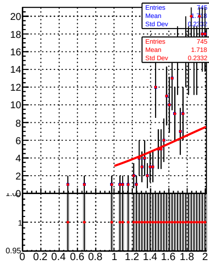
Raw Jet response (pT/pTgen) in 15 \leq p_t < 21, 3.0 \leq |\eta| < 5.0
