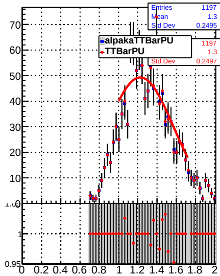
Raw Jet response (pT/pTgen) in 15 \leq p_t < 21, 0.0 \leq |\eta| < 0.5
