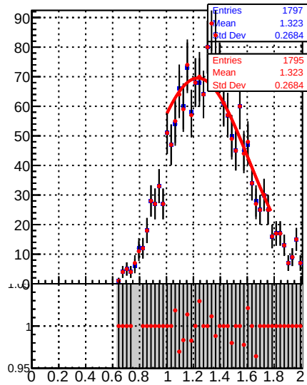
Raw Jet response (pT/pTgen) in 15 \leq p_t < 21, 0.5 \leq |\eta| < 2.1
