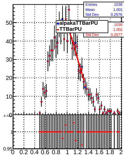
Jet response ( pT/pT_{\text{gen}} ) in 15 \leq p_t < 21 , 0.5 \leq |\eta| < 0.5
