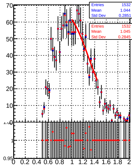
Jet response ( pT/pT_{\text{gen}} ) in 15 \leq p_t < 21 , 0.5 \leq |\eta| < 1.3
