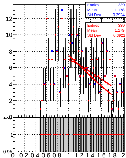
Jet response ( pT/pT_{\text{gen}} ) in 15 \leq p_t < 21 , 2.5 \leq |\eta| < 3.0
