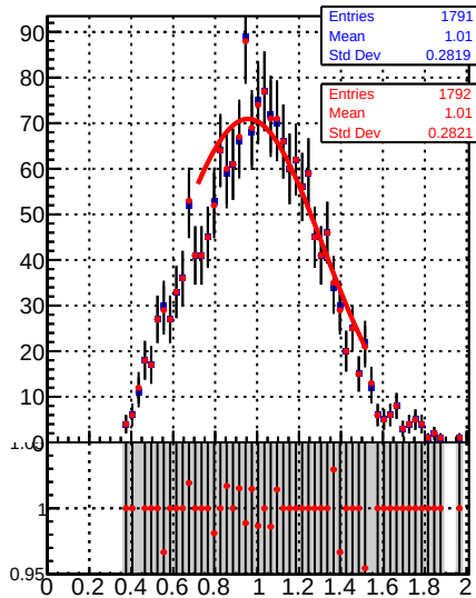
Jet response ( pT/pT_{\text{gen}} ) in 21 \leq p_t < 28, 0.5 \leq |\eta| < 2.1
