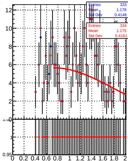
Jet response ( pT/pT_{\text{gen}} ) in 21 \leq p_t < 28, 2.5 \leq |\eta| < 3.0
