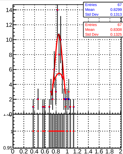
Raw Jet response (pT/pTgen) in 153 &lt;= pt &lt; 196, 2.1 &lt;= |eta| &lt; 2.5
