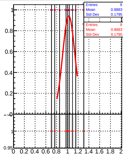
Raw Jet response (pT/pTgen) in 153 &lt;= pt &lt; 196, 3.0 &lt;= |eta| &lt; 5.0
