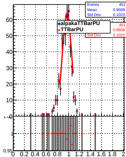
Raw Jet response (pT/pTgen) in 153 &lt;= pt &lt; 196, 0.0 &lt;= |eta| &lt; 0.5
