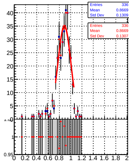
Raw Jet response (pT/pTgen) in 153 &lt;= pt &lt; 196, 1.3 &lt;= |eta| &lt; 2.1
