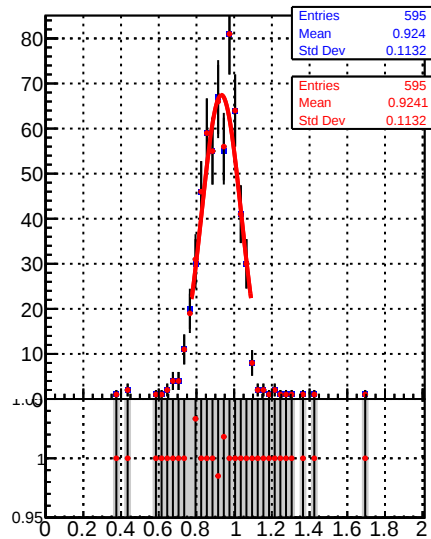
Raw Jet response (pT/pTgen) in 153 &lt;= pt &lt; 196, 0.5 &lt;= |eta| &lt; 1.3
