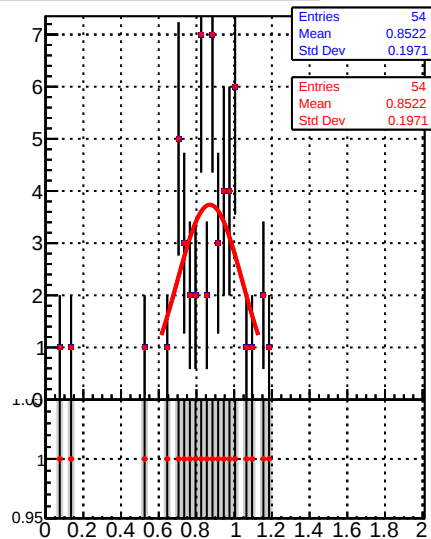
Raw Jet response (pT/pTgen) in 153 &lt;= pt &lt; 196, 2.5 &lt;= |eta| &lt; 3.0
