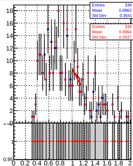
Raw Jet response (pT/pTgen) in 15 &lt;= pt &lt; 21, 2.5 &lt;= |eta| &lt; 3.0
