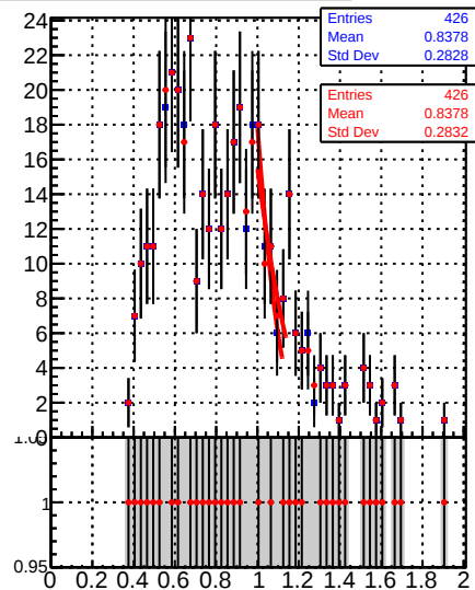
Raw Jet response (pT/pTgen) in 15 &lt;= pt &lt; 21, 2.1 &lt;= |eta| &lt; 2.5
