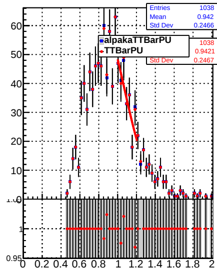
Raw Jet response (pT/pTgen) in 15 &lt;= pt &lt; 21, 0.0 &lt;= |eta| &lt; 0.5
