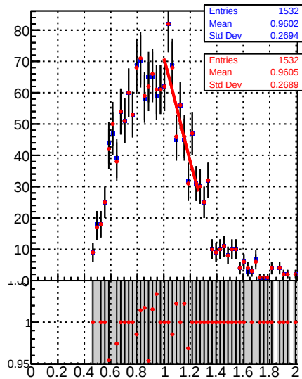
Raw Jet response (pT/pTgen) in 15 &lt;= pt &lt; 21, 0.5 &lt;= |eta| &lt; 1.3
