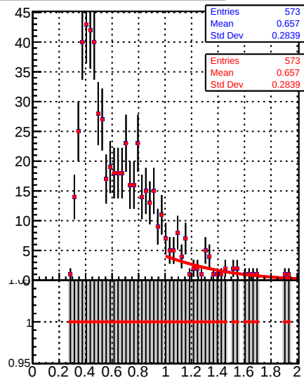
Raw Jet response (pT/pTgen) in 15 &lt;= pt &lt; 21, 3.0 &lt;= |eta| &lt; 5.0
