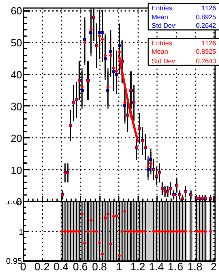
Raw Jet response (pT/pTgen) in 15 &lt;= pt &lt; 21, 1.3 &lt;= |eta| &lt; 2.1
