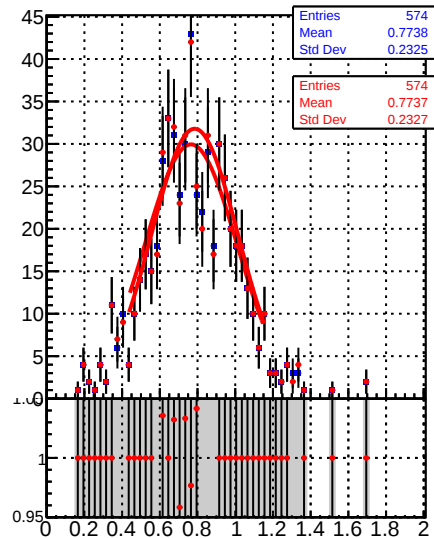
Raw Jet response (pT/pTgen) in 37 \leq p_t < 49, 2.1 \leq |\eta| < 2.5
