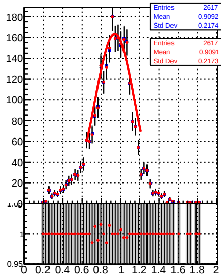
Raw Jet response (pT/pTgen) in 37 \leq p_t < 49, 0.5 \leq |\eta| < 1.3
