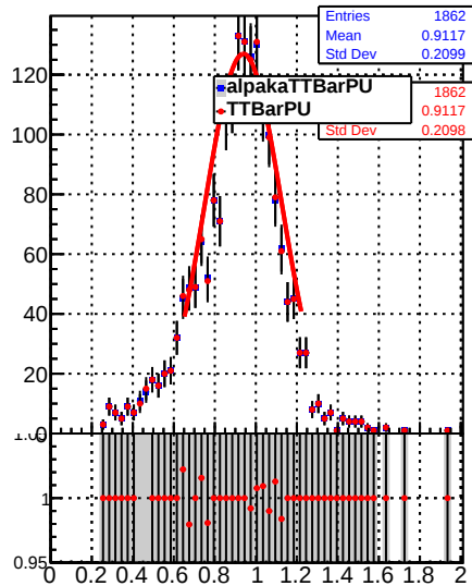
Raw Jet response (pT/pTgen) in 37 \leq p_t < 49, 0.0 \leq |\eta| < 0.5
