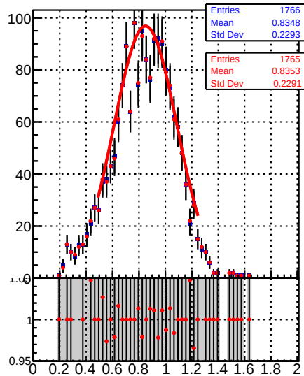
Raw Jet response (pT/pTgen) in 37 \leq p_t < 49, 1.3 \leq |\eta| < 2.1
