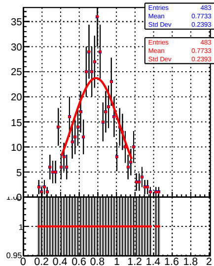
Raw Jet response (pT/pTgen) in 37 \leq p_t < 49, 3.0 \leq |\eta| < 5.0
