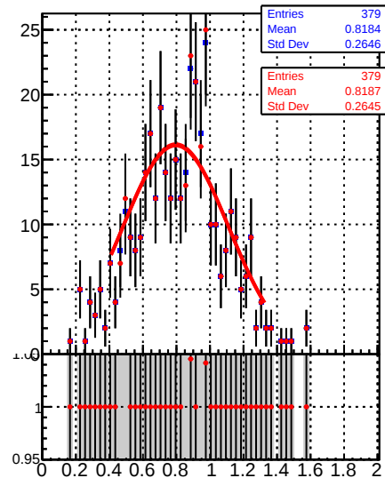
Raw Jet response (pT/pTgen) in 37 \leq p_t < 49, 2.5 \leq |\eta| < 3.0
