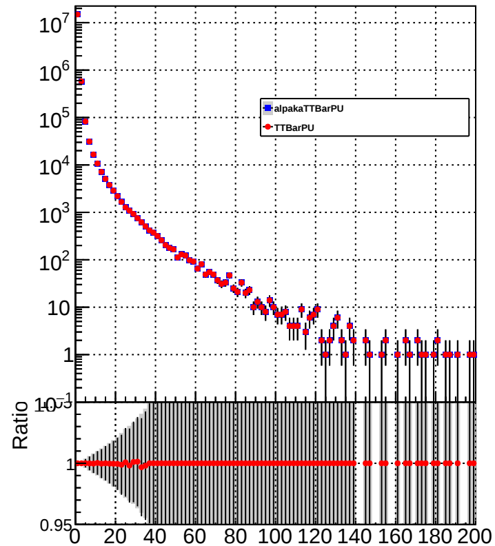
chargedHadronPtMid
