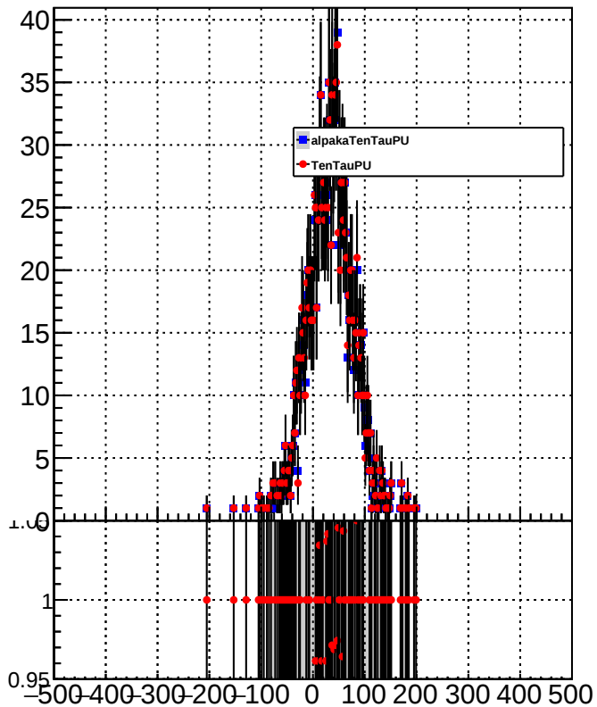
METResolution_GenMETTrue_MET200to300
