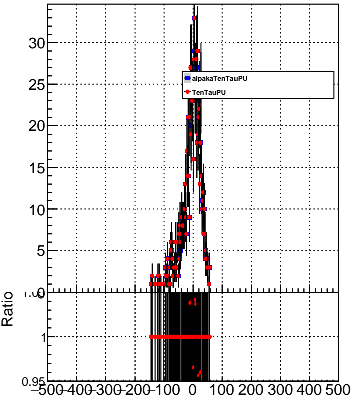
METResolution_GenMETtrue_MET40to60
