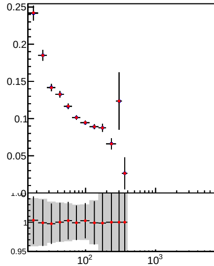
Jet pT resolution, 1.3 < |\eta| < 2.1
