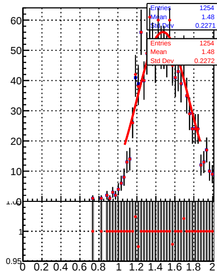
Raw Jet response (pT/pTgen) in 15 &lt;= pt &lt; 21, 0.5 &lt;= |eta| &lt; 1.3
