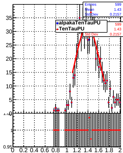
Raw Jet response (pT/pTgen) in 15 &lt;= pt &lt; 21, 0.0 &lt;= |eta| &lt; 1.3
