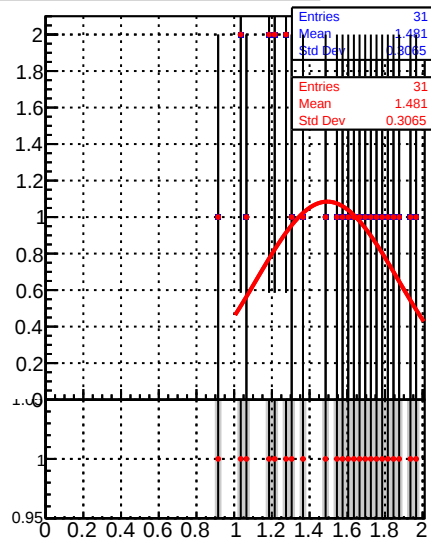
Raw Jet response (pT/pTgen) in 15 &lt;= pt &lt; 21, 2.5 &lt;= |eta| &lt; 3.0
