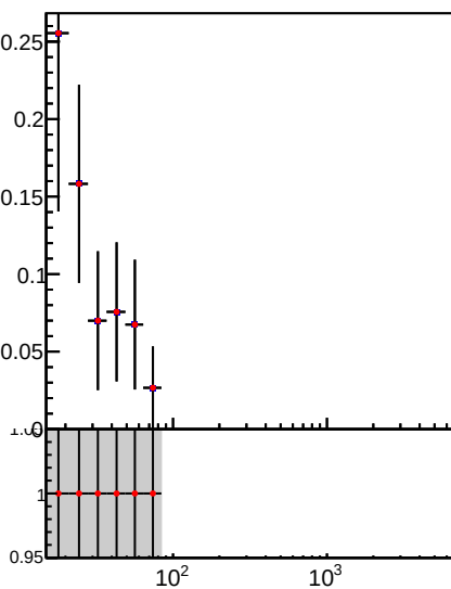
Raw Jet pT resolution, 2.5 < |\eta| < 3.0
