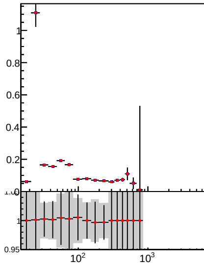
Raw Jet pT resolution, 0.5 < |\eta| < 1.3
