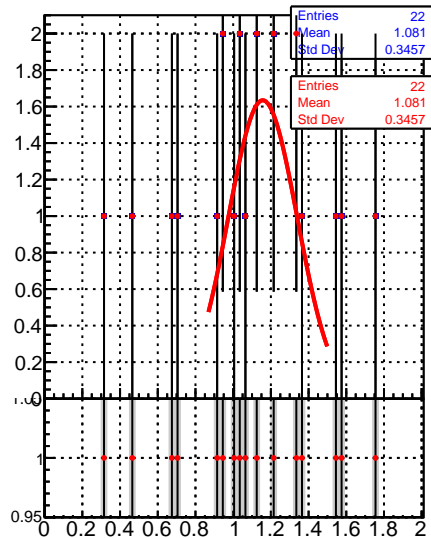
Raw Jet response (pT/pTgen) in 21 &lt;math&gt;\leq p_t &lt; 28, 2.5 \leq |\eta| &lt; 3.0&lt;/math&gt;
