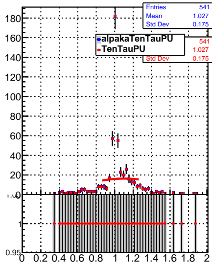
Raw Jet response (pT/pTgen) in 21 &lt;math&gt;\leq p_t &lt; 28, 0.0 \leq |\eta| &lt; 0.5&lt;/math&gt;
