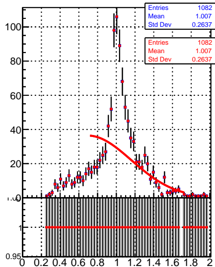
Raw Jet response (pT/pTgen) in 21 &lt;math&gt;\leq p_t &lt; 28, 2.1 \leq |\eta| &lt; 2.5&lt;/math&gt;
