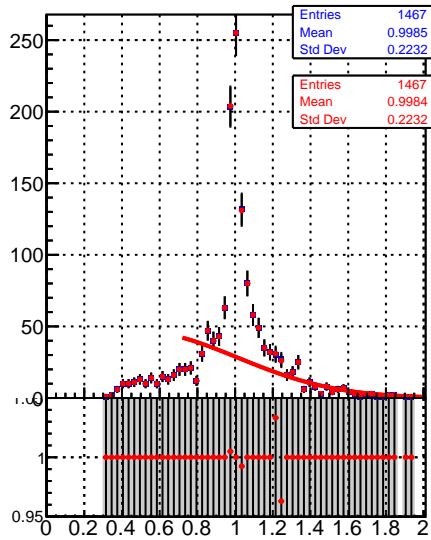
Raw Jet response (pT/pTgen) in 21 &lt;math&gt;\leq p_t &lt; 28, 1.3 \leq |\eta| &lt; 2.1&lt;/math&gt;
