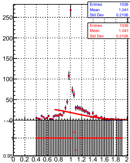
Raw Jet response (pT/pTgen) in 21 &lt;math&gt;\leq p_t &lt; 28, 0.5 \leq |\eta| &lt; 1.3&lt;/math&gt;
