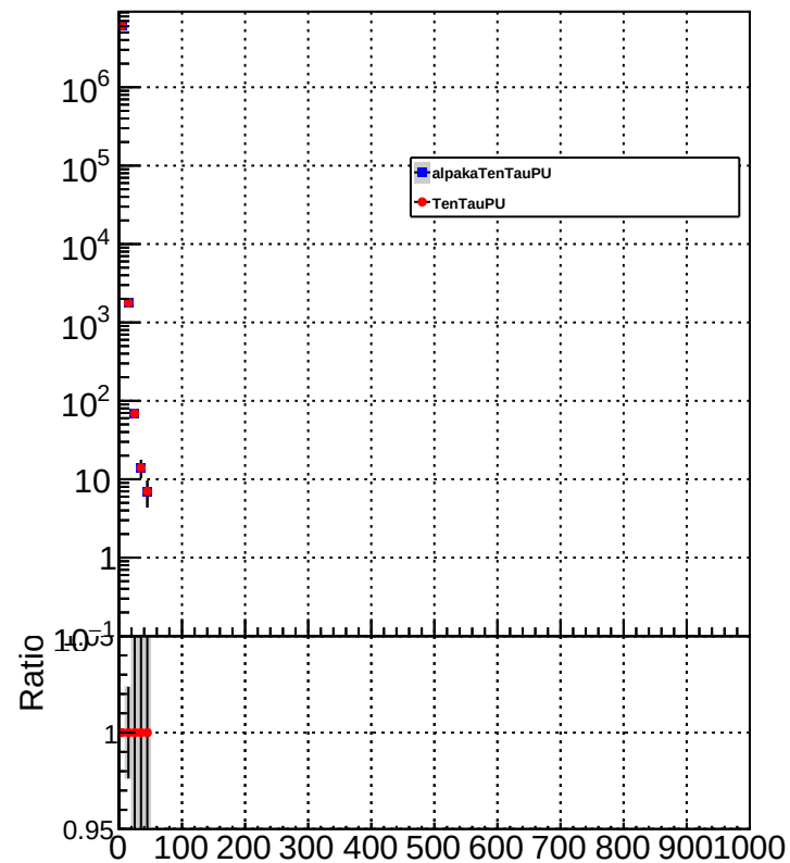
HF_hadronPtHigh
