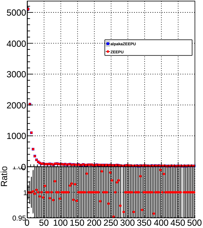
neutralHadronEnergy
