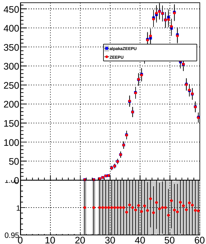
number of vertices
