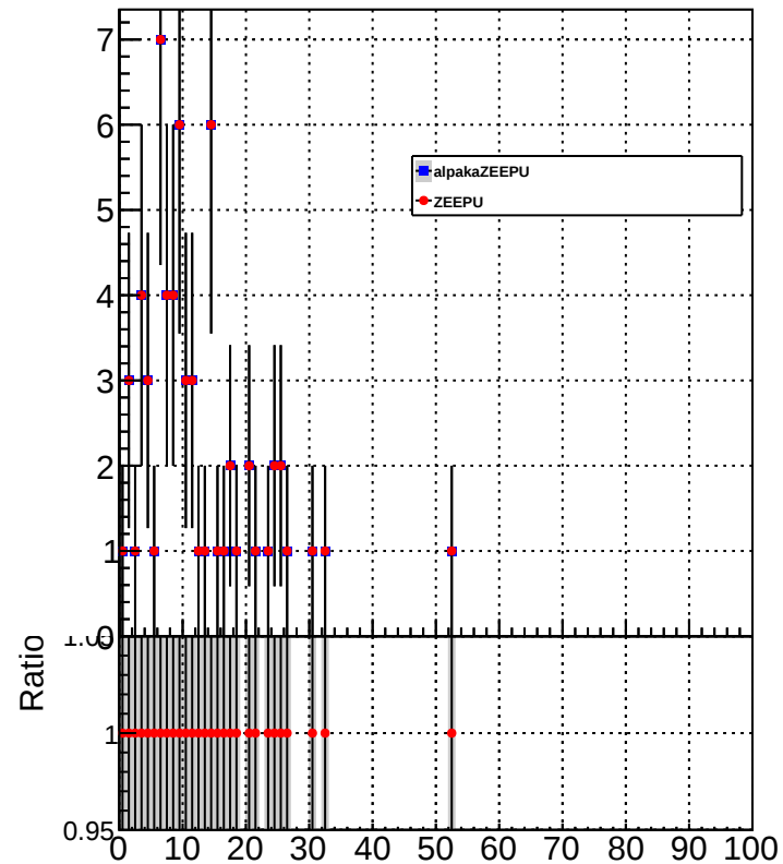
chargedMultiplicity
