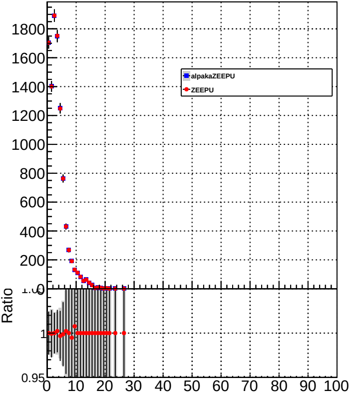
chargedMultiplicity
