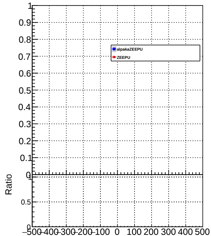
METResolution_GenMETTrue_MET200to300
