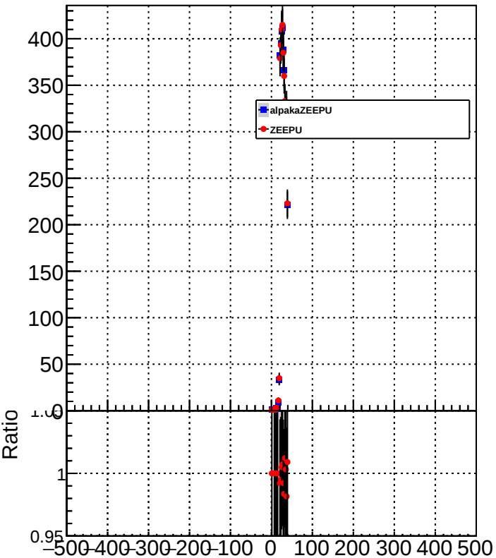
METResolution_GenMETTrue_MET20to40
