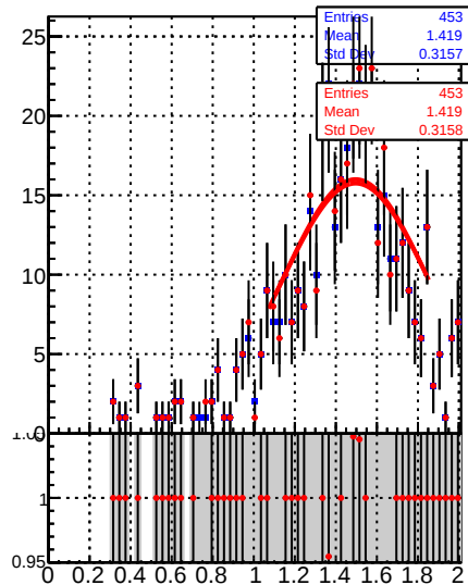
Jet response (pT/pTgen) in 28 \leq pt < 37, 2.5 \leq |\eta| < 3.0
