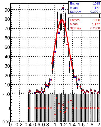
Jet response (pT/pTgen) in 28 \leq pt < 37, 0.5 \leq |\eta| < 1.3
