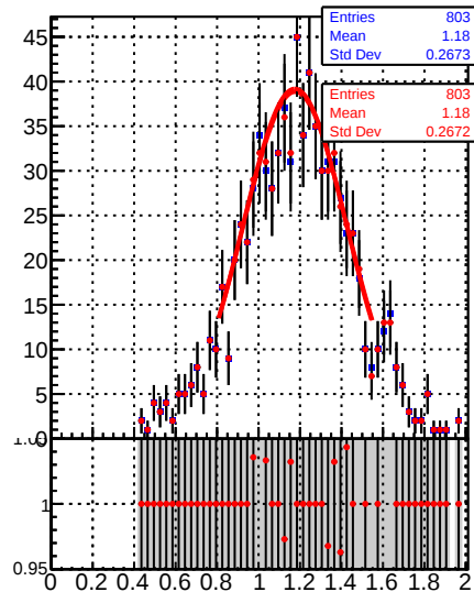
Jet response (pT/pTgen) in 28 \leq pt < 37, 3.0 \leq |\eta| < 5.0
