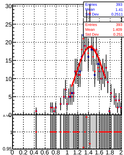
Jet response (pT/pTgen) in 28 \leq pt < 37, 2.1 \leq |\eta| < 2.5
