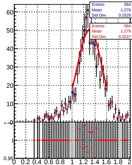
Jet response (pT/pTgen) in 28 \leq pt < 37, 1.3 \leq |\eta| < 2.1
