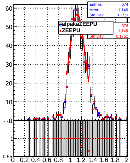
Jet response (pT/pTgen) in 28 \leq pt < 37, 0.0 \leq |\eta| < 1.3
