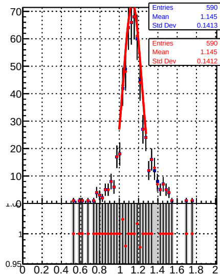
Jet response (pT/pTgen) in 49 \leq p_t < 64 , 0.5 \leq |\eta| < 2.1
