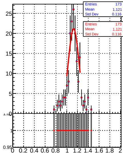
Jet response (pT/pTgen) in 64 \leq p_t < 84 , 0.5 \leq |\eta| < 1.3
