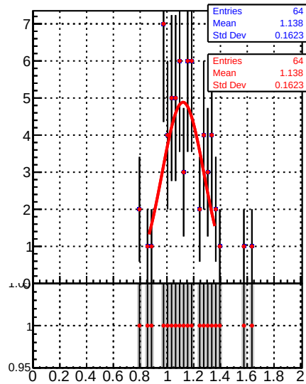
Jet response (pT/pTgen) in 64 \leq p_t < 84 , 3.0 \leq |\eta| < 5.0
