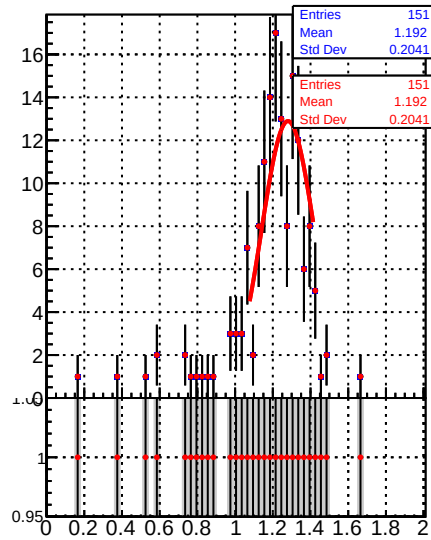
Jet response (pT/pTgen) in 64 \leq p_t < 84 , 1.3 \leq |\eta| < 2.1
