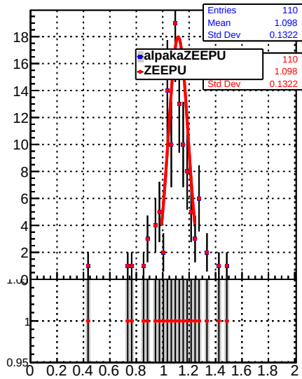
Jet response (pT/pTgen) in 64 \leq p_t < 84 , 0.0 \leq |\eta| < 0.5
