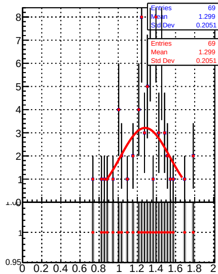
Jet response (pT/pTgen) in 64 \leq p_t < 84 , 2.5 \leq |\eta| < 3.0
