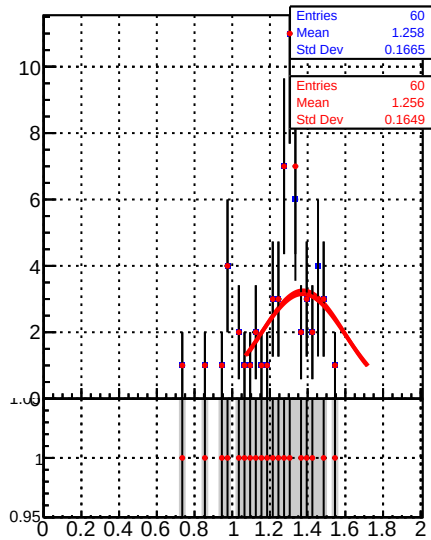
Jet response (pT/pTgen) in 64 \leq p_t < 84 , 2.1 \leq |\eta| < 2.5
