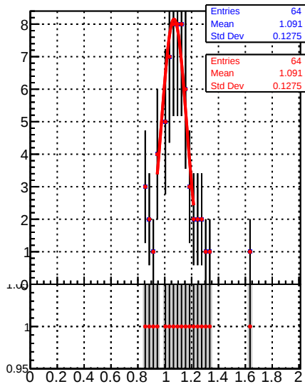
Jet response ( p_T/p_{T\text{gen}} ) in 84 \leq p_t < 114 , 0.5 \leq |\eta| < 1.3
