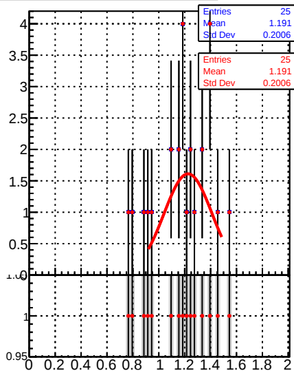
Jet response ( p_T/p_{T\text{gen}} ) in 84 \leq p_t < 114 , 2.5 \leq |\eta| < 3.0
