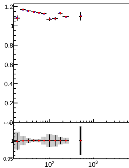
Jet pT response, 0.5 < |\eta| < 1.3
