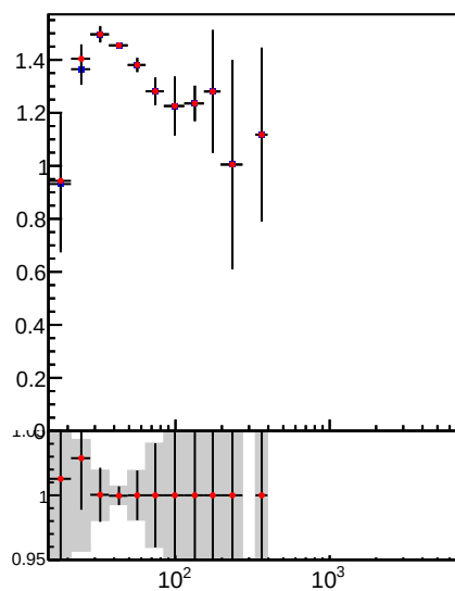
Jet pT response, 2.5 < |\eta| < 3.0
