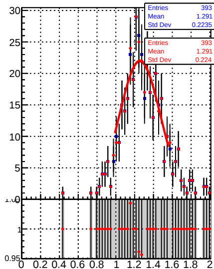
Raw Jet response (pT/pTgen) in 28 \leq p_t < 37 , 2.1 \leq |\eta| < 2.5
