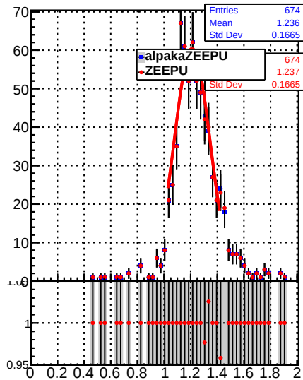
Raw Jet response (pT/pTgen) in 28 \leq p_t < 37 , 0.0 \leq |\eta| < 2.1
