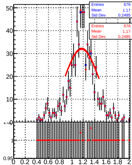
Jet response (pT/pTgen) in 21 \leq p_t < 28, 0.5 \leq |\eta| < 1.3
