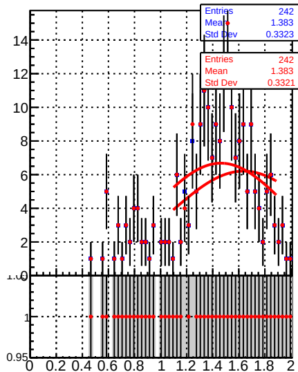
Jet response (pT/pTgen) in 21 \leq p_t < 28, 2.1 \leq |\eta| < 2.5
