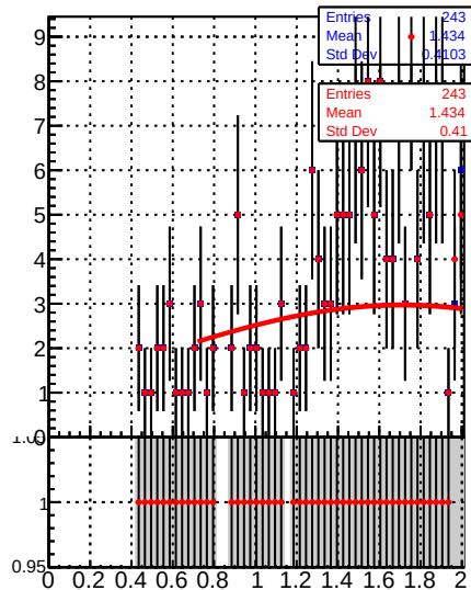
Jet response (pT/pTgen) in 21 \leq p_t < 28, 2.5 \leq |\eta| < 3.0
