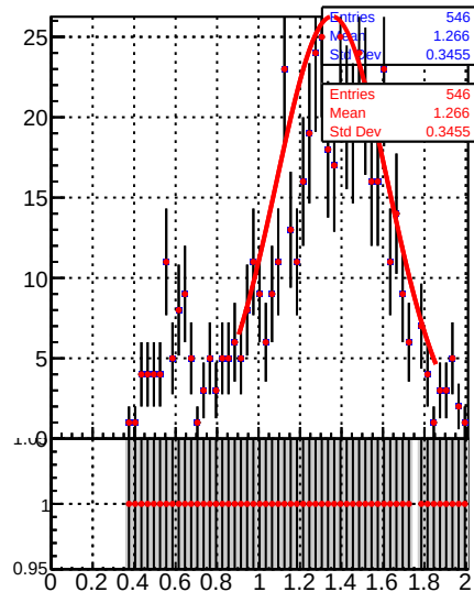
Jet response (pT/pTgen) in 21 \leq p_t < 28, 3.0 \leq |\eta| < 5.0
