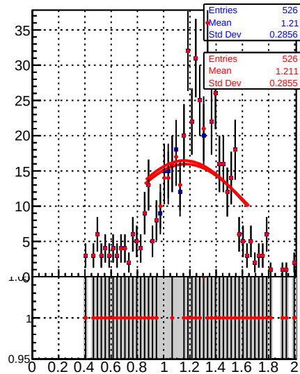
Jet response (pT/pTgen) in 21 \leq p_t < 28, 1.3 \leq |\eta| < 2.1
