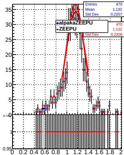
Jet response (pT/pTgen) in 21 \leq p_t < 28, 0.0 \leq |\eta| < 0.5
