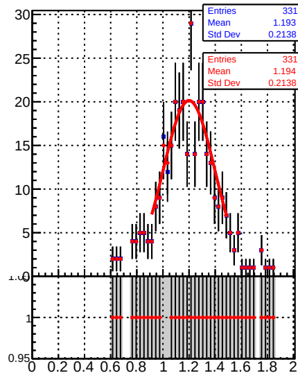
Jet response (pT/pTgen) in 49 \leq pt < 64, 3.0 \leq |\eta| < 5.0
