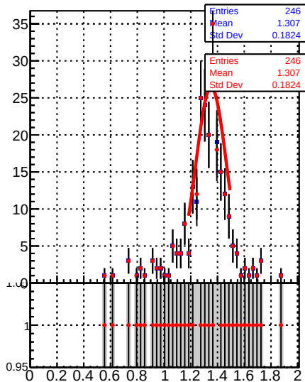
Jet response (pT/pTgen) in 49 \leq pt < 64, 2.1 \leq |\eta| < 2.5
