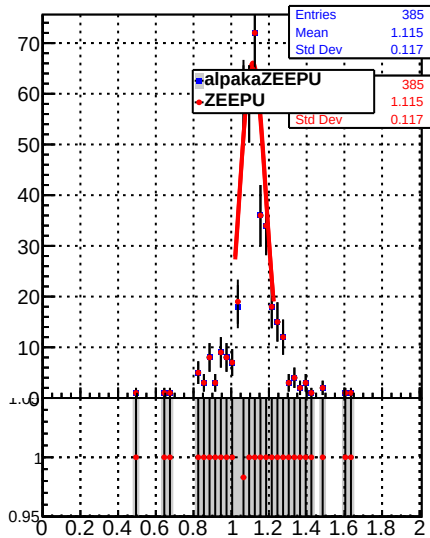
Jet response (pT/pTgen) in 49 \leq pt < 64, 0.0 \leq |\eta| < 0.5
