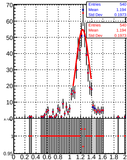
Jet response (pT/pTgen) in 49 \leq pt < 64, 1.3 \leq |\eta| < 2.1
