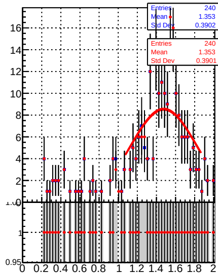
Jet response (pT/pTgen) in 49 \leq pt < 64, 2.5 \leq |\eta| < 3.0
