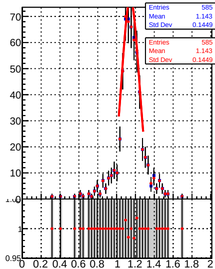
Jet response (pT/pTgen) in 49 \leq pt < 64, 0.5 \leq |\eta| < 1.3
