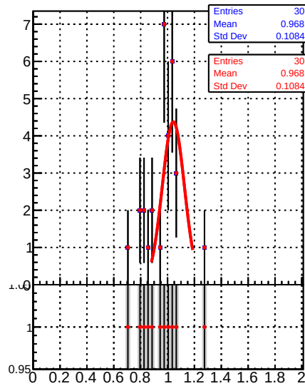
Raw Jet response (pT/pTgen) in 114 &lt;= pt &lt; 153, 1.3 &lt;= |eta| &lt; 2.1
