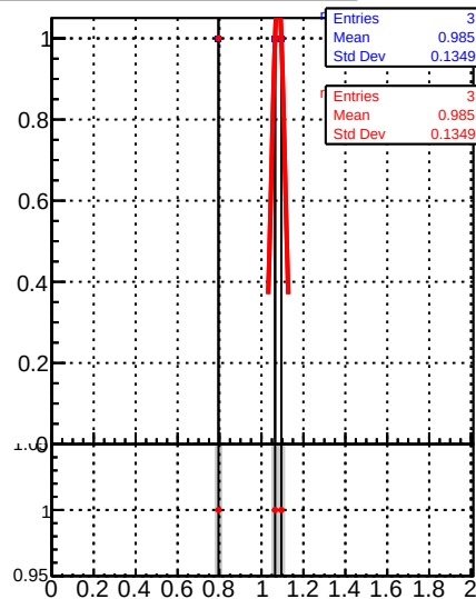
Raw Jet response (pT/pTgen) in 114 &lt;= pt &lt; 153, 3.0 &lt;= |eta| &lt; 5.0
