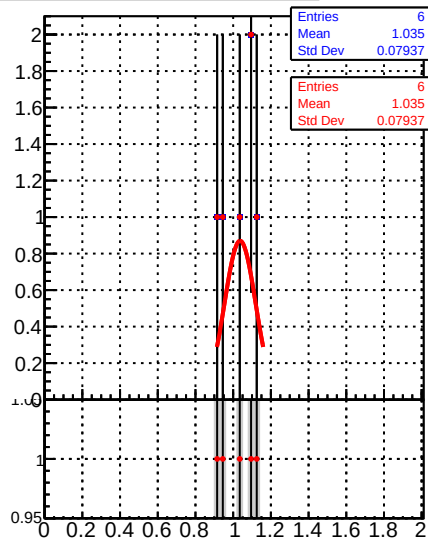
Raw Jet response (pT/pTgen) in 114 &lt;= pt &lt; 153, 2.5 &lt;= |eta| &lt; 3.0
