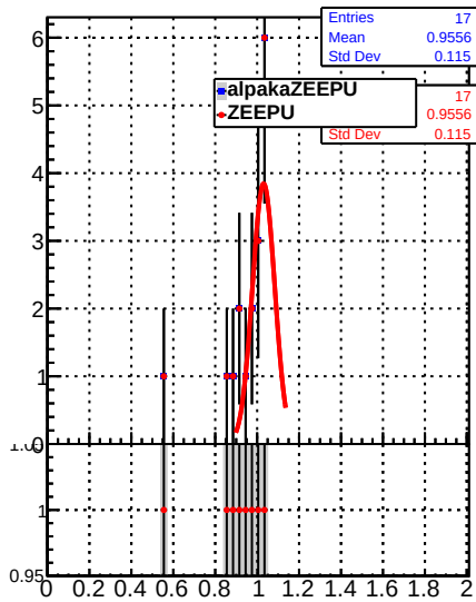
Raw Jet response (pT/pTgen) in 114 &lt;= pt &lt; 153, 0.0 &lt;= |eta| &lt; 0.5
