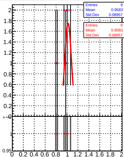
Raw Jet response (pT/pTgen) in 114 &lt;= pt &lt; 153, 2.1 &lt;= |eta| &lt; 2.5
