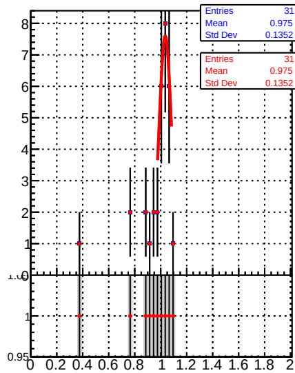
Raw Jet response (pT/pTgen) in 114 &lt;= pt &lt; 153, 0.5 &lt;= |eta| &lt; 1.3
