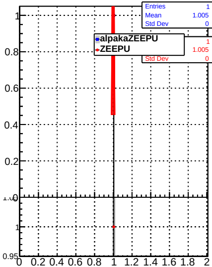
Raw Jet response (pT/pTgen) in 272 &lt;= pt &lt; 330, 0.0 &lt;= |eta| &lt; 0.5
