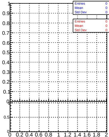
Raw Jet response (pT/pTgen) in 272 &lt;= pt &lt; 330, 2.1 &lt;= |eta| &lt; 2.5
