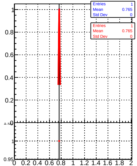
Raw Jet response (pT/pTgen) in 272 &lt;= pt &lt; 330, 1.3 &lt;= |eta| &lt; 2.1
