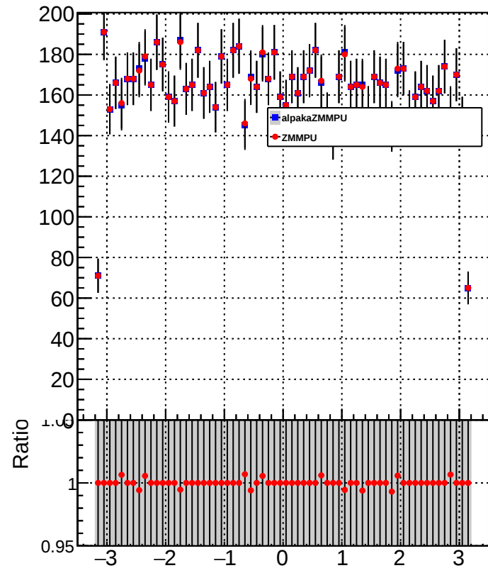
CorrJetPhi Pt>40
