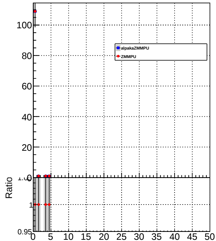
HFHadronMultiplicity
