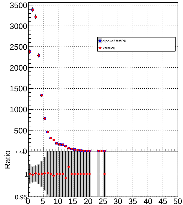
chargedHadronMultiplicity
