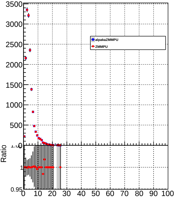
chargedMultiplicity
