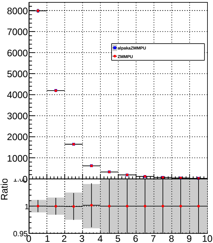
photonMultiplicity
