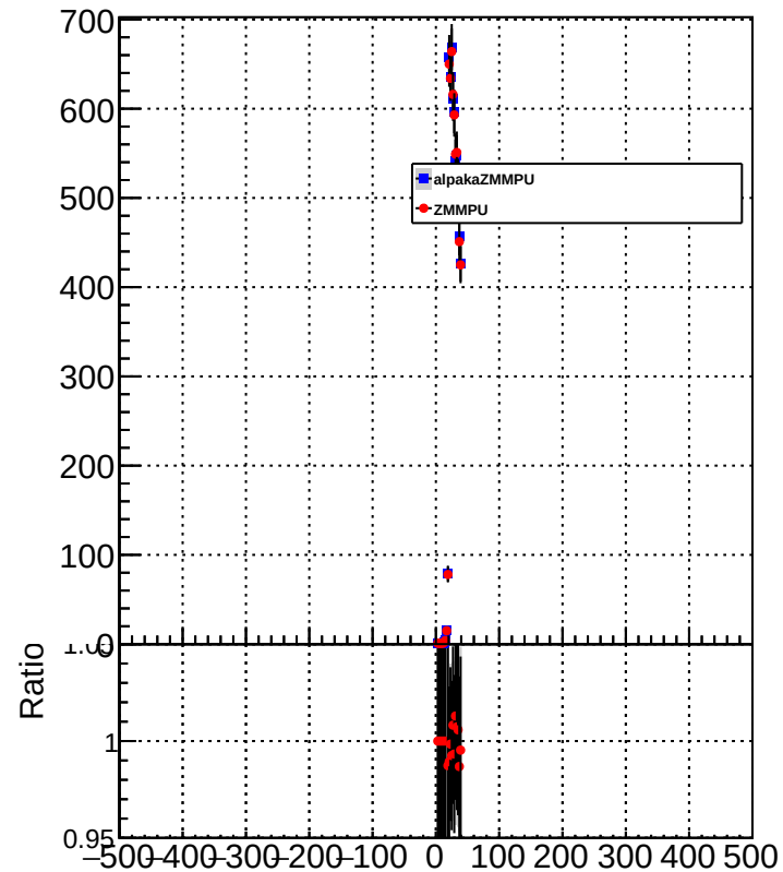
METResolution_GenMETTrue_MET20to40
