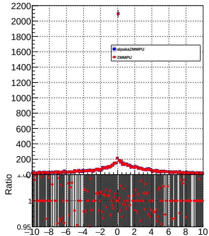
METUnc_JetResDown
