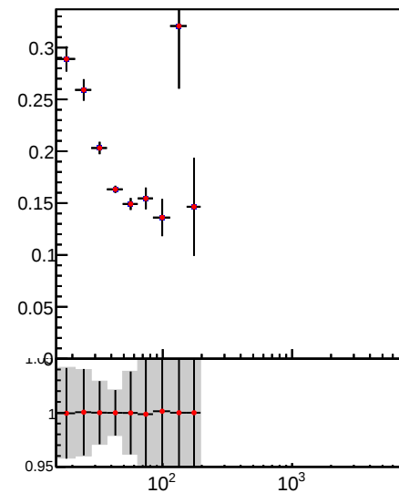
Jet pT resolution using RMS, 2.1 < |\eta| < 2.5
