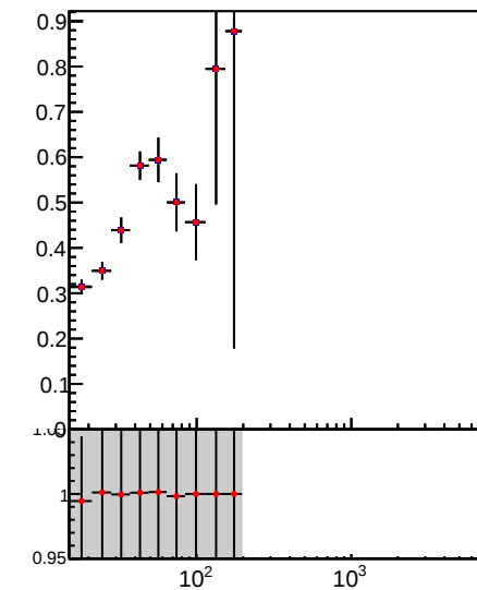
Jet pT resolution using RMS, 2.5 < |\eta| < 3.0
