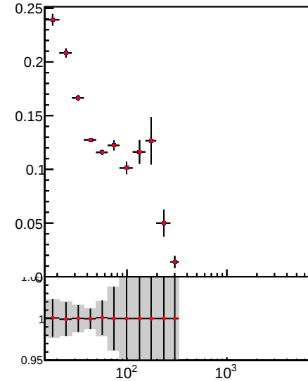
Jet pT resolution using RMS, 0.5 < |\eta| < 1.3
