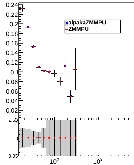
Jet pT resolution using RMS, 0.0 < |\eta| < 0.5
