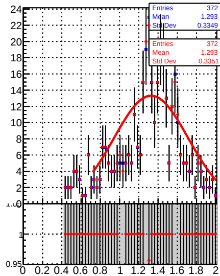
Jet response ( p_T/p_{Tgen} ) in 21 \leq pt < 28, 2.1 \leq |\eta| < 2.5
