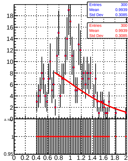
Jet response ( p_T/p_{Tgen} ) in 21 \leq pt < 28, 3.0 \leq |\eta| < 5.0
