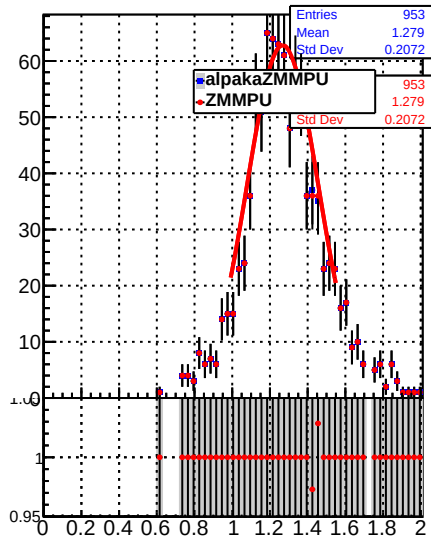
Raw Jet response (pT/pTgen) in 21 &lt;= pt &lt; 28, 0.0 &lt;= |eta| &lt; 1.3
