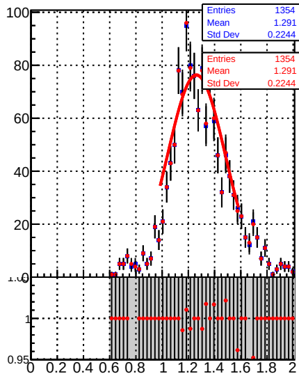
Raw Jet response (pT/pTgen) in 21 &lt;= pt &lt; 28, 0.5 &lt;= |eta| &lt; 1.3
