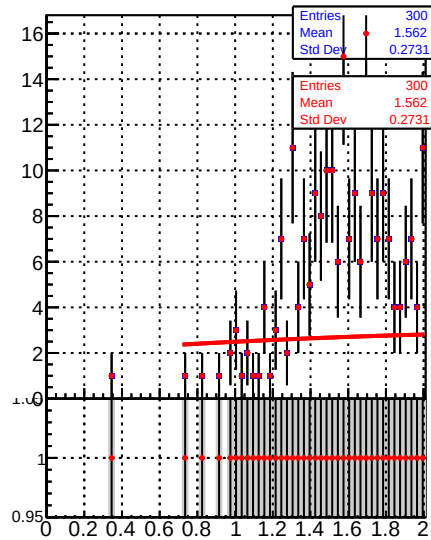
Raw Jet response (pT/pTgen) in 21 &lt;= pt &lt; 28, 3.0 &lt;= |eta| &lt; 5.0
