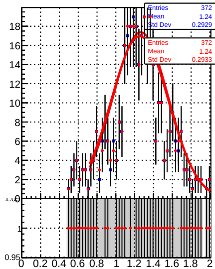
Raw Jet response (pT/pTgen) in 21 &lt;= pt &lt; 28, 2.1 &lt;= |eta| &lt; 2.5
