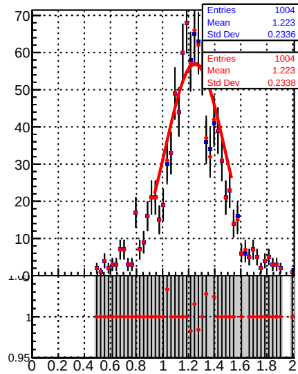
Raw Jet response (pT/pTgen) in 21 &lt;= pt &lt; 28, 1.3 &lt;= |eta| &lt; 2.1
