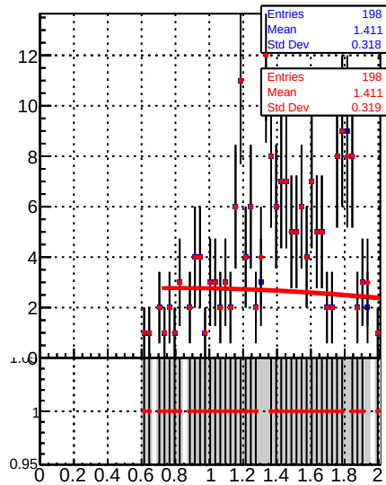
Raw Jet response (pT/pTgen) in 21 &lt;= pt &lt; 28, 2.5 &lt;= |eta| &lt; 3.0
