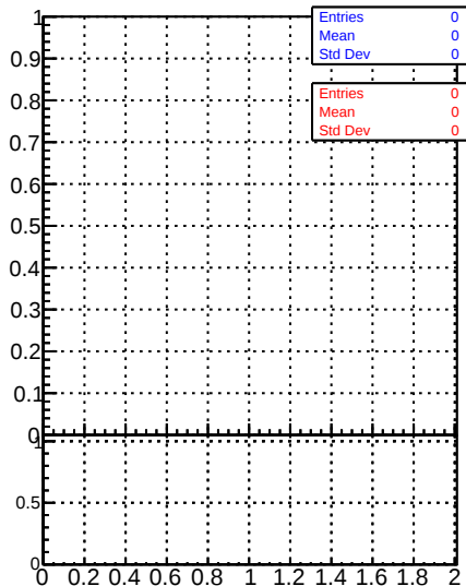
Raw Jet response (pT/pTgen) in 468 &lt;= pt &lt; 548, 2.1 &lt;= |eta| &lt; 2.5
