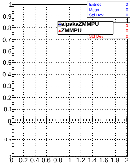
Raw Jet response (pT/pTgen) in 468 &lt;= pt &lt; 548, 0.0 &lt;= |eta| &lt; 0.5
