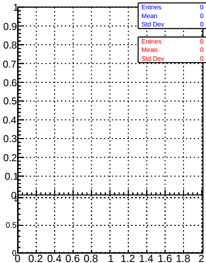
Raw Jet response (pT/pTgen) in 468 &lt;= pt &lt; 548, 0.5 &lt;= |eta| &lt; 1.3
