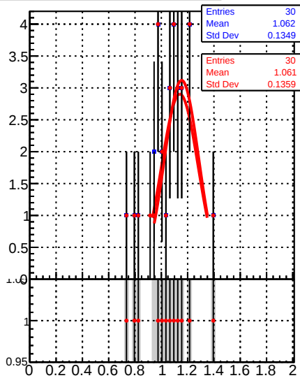
Raw Jet response (pT/pTgen) in 84 &lt;= pt &lt; 114, 2.1 &lt;= |eta| &lt; 2.5
