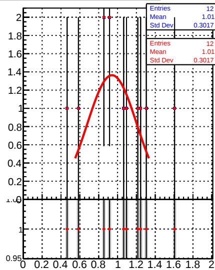
Raw Jet response (pT/pTgen) in 84 &lt;= pt &lt; 114, 3.0 &lt;= |eta| &lt; 5.0
