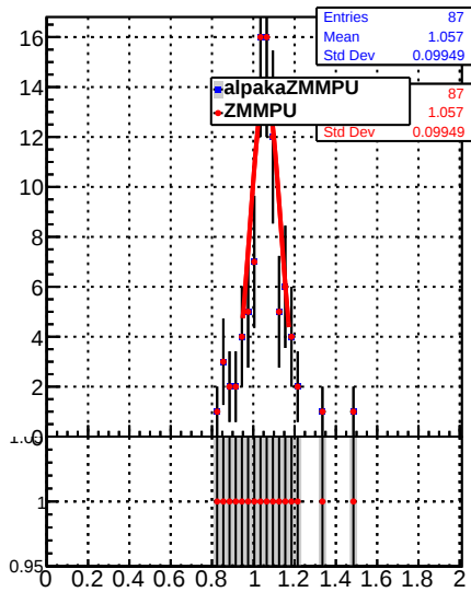
Raw Jet response (pT/pTgen) in 84 &lt;= pt &lt; 114, 0.0 &lt;= |eta| &lt; 0.5
