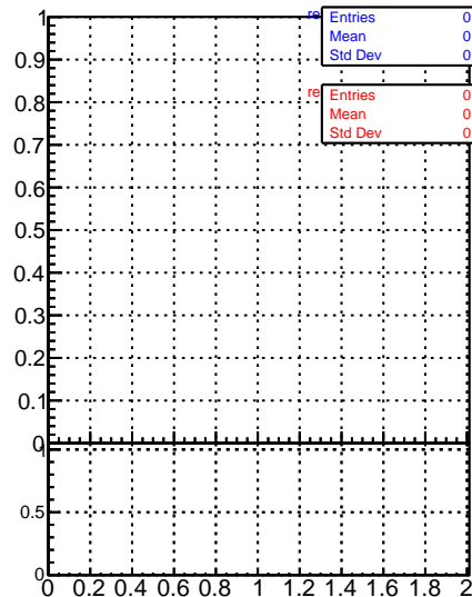
Jet response (pT/pTgen) in 1248 <math>\leq pt < 1588, 3.0 \leq |\eta| < 5.0</math>
