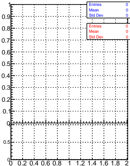
Jet response (pT/pTgen) in 1248 <math>\leq pt < 1588, 0.5 \leq |\eta| < 1.3</math>
