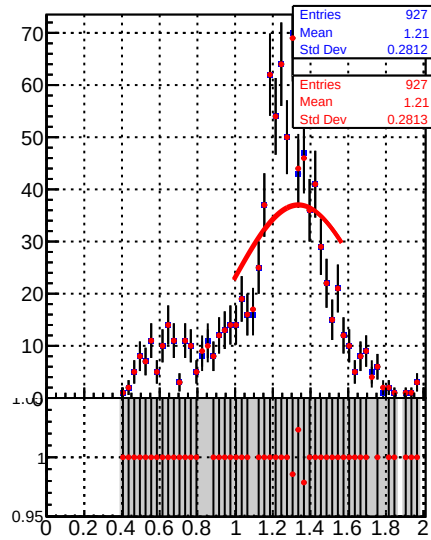
Jet response (pT/pTgen) in 21 \leq pt < 28, 1.3 \leq |\eta| < 2.1
