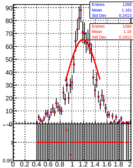
Jet response (pT/pTgen) in 21 \leq pt < 28, 0.5 \leq |\eta| < 1.3
