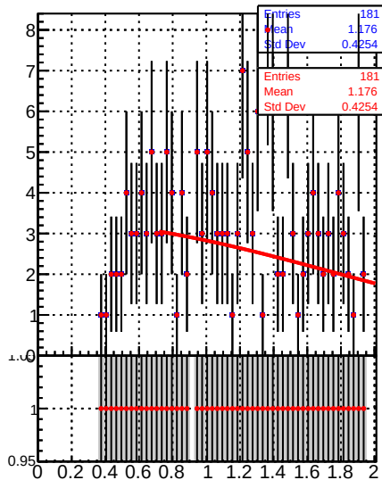
Jet response (pT/pTgen) in 21 \leq pt < 28, 2.5 \leq |\eta| < 3.0
