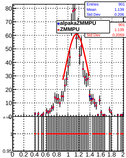
Jet response (pT/pTgen) in 21 \leq pt < 28, 0.0 \leq |\eta| < 0.5
