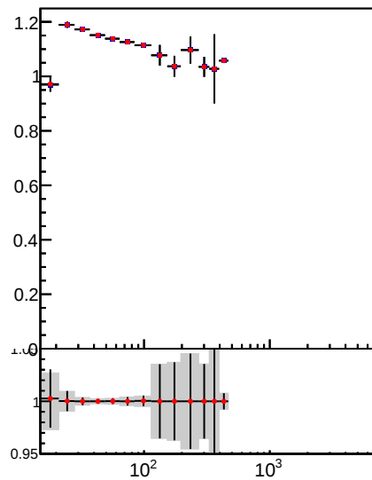
Jet pT response, 0.5 < |\eta| < 1.3
