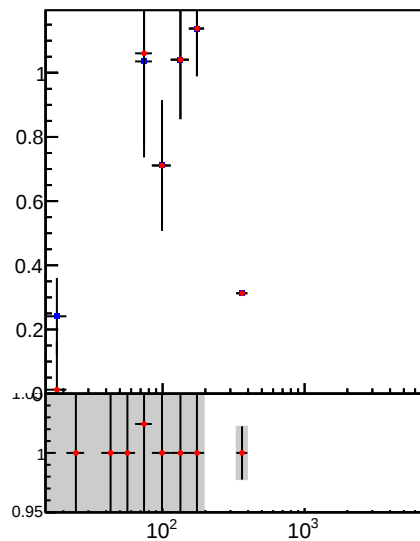
Jet pT response, 2.5 < |\eta| < 3.0
