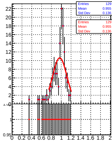
Raw Jet response (pT/pTgen) in 84 &lt;= pt &lt; 114, 1.3 &lt;= |eta| &lt; 2.1
