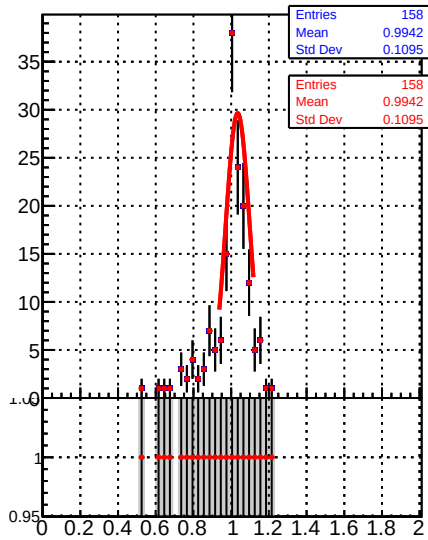
Raw Jet response (pT/pTgen) in 84 &lt;= pt &lt; 114, 0.5 &lt;= |eta| &lt; 1.3
