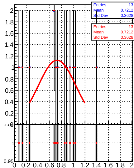
Raw Jet response (pT/pTgen) in 84 &lt;= pt &lt; 114, 3.0 &lt;= |eta| &lt; 5.0
