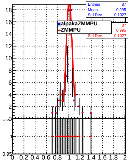
Raw Jet response (pT/pTgen) in 84 &lt;= pt &lt; 114, 0.0 &lt;= |eta| &lt; 2.5
