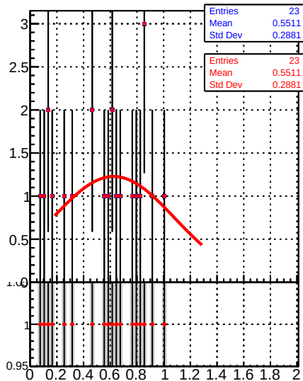
Raw Jet response (pT/pTgen) in 84 &lt;= pt &lt; 114, 2.5 &lt;= |eta| &lt; 3.0
