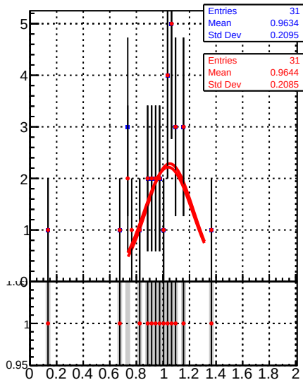
Raw Jet response (pT/pTgen) in 84 &lt;= pt &lt; 114, 2.1 &lt;= |eta| &lt; 2.5
